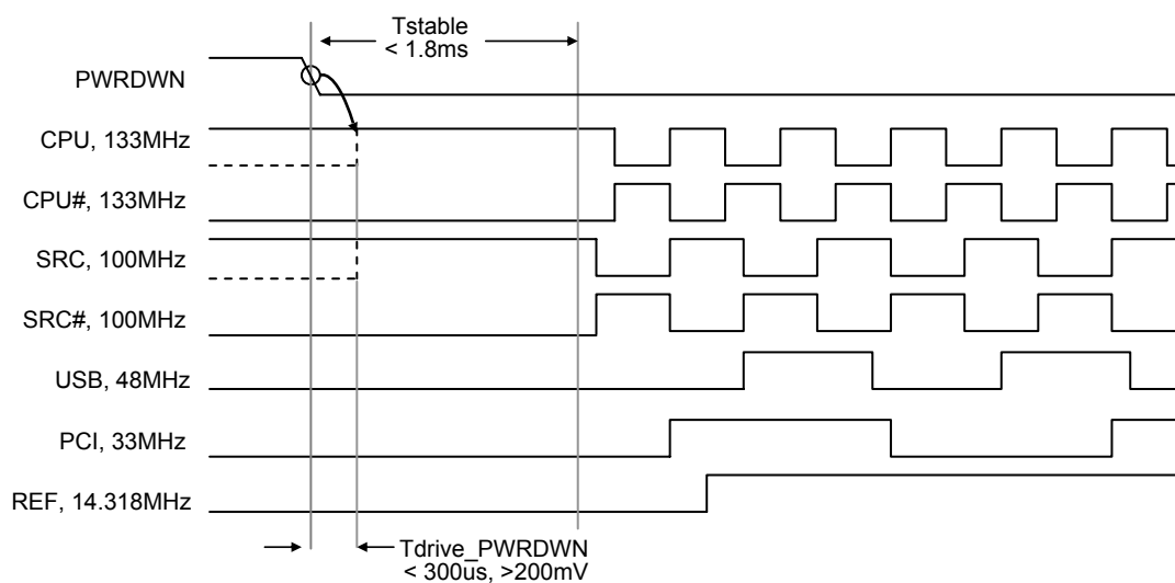
Figure 2. Power down de-assert sequence
