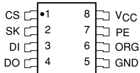
SOIC Package (S,V)
