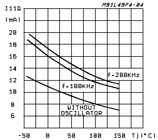
Figure 9 : Quiescent Drain Current vs. Junction Temperature (0% duty cycle).
