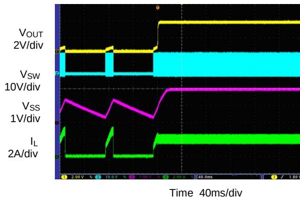
Short Circuit Recovery ( I_{OUT}=2\text{A} )
