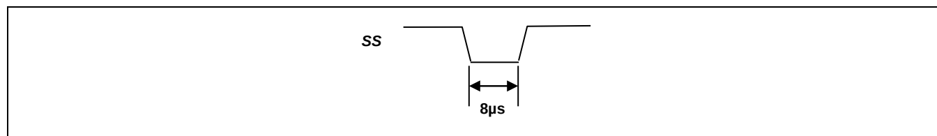
Figure 3.7 SPI Read_MR
