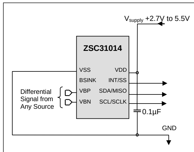
Figure 4.2 Example 2 Circuit Diagram: Generic Differential A2D Converter
