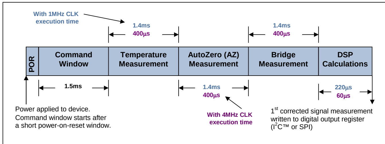
Figure 3.2 Power-Up Sequence and Timing for Update Mode with EEPROM Locked s
