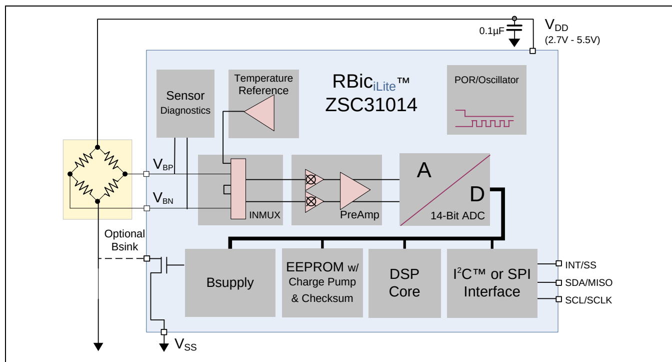
Figure 2.1 ZSC31014 Block Diagram
