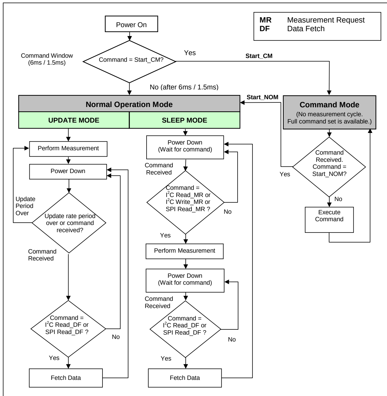
Figure 3.1 General Working Mode
