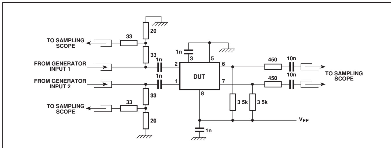
Fig. 5 Test circuit
