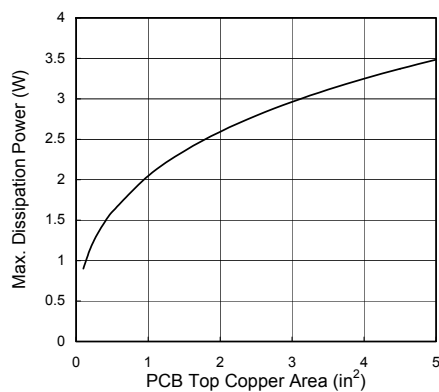
G1085T43(TO-252) Max. Power Dissipation vs. PCB Top Copper Area Area T_{AMB} = 25^{\circ}\text{C} ; Still Air
