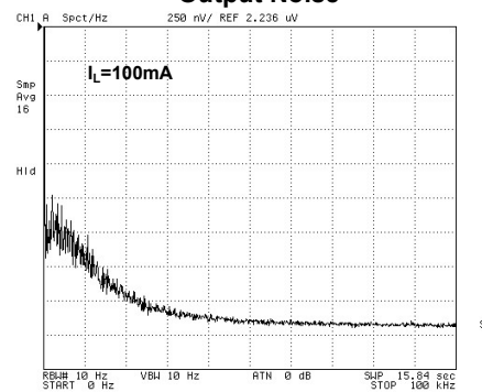
Output Noise
