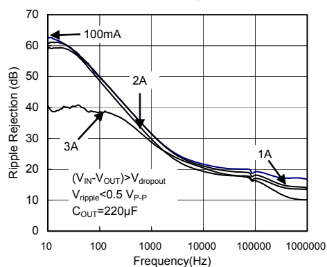
Ripple Rejection
