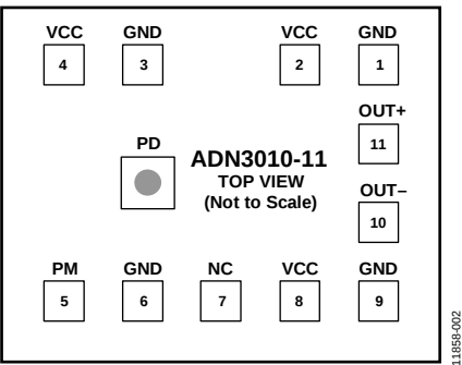
Figure 2. Pad Configuration
