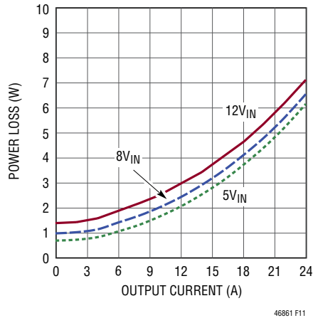
Figure 11. 1V OUT Power Loss Curve
