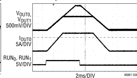
FIGURE 61 CIRCUIT AT 12\text{V}_{\text{IN}} , 100\text{m}\Omega LOAD ON \text{V}_{\text{OUT}0} . NO LOAD ON \text{V}_{\text{OUT}1} . \text{TON\_RISE}_0 = 3\text{ms} , \text{TON\_RISE}_1 = 5.297\text{ms} , \text{TOFF\_DELAY}_1 = 0\text{ms} , \text{TOFF\_DELAY}_0 = 2.43\text{ms} , \text{TOFF\_FALL}_1 = 5.328\text{ms} , \text{TOFF\_FALL}_0 = 3\text{ms} , \text{ON\_OFF\_CONFIG}_n = 0\text{x}1\text{E}
