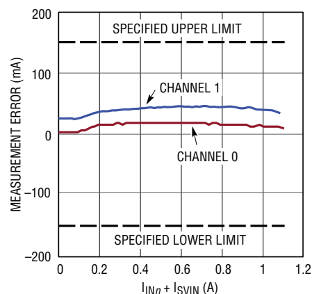
MFR_READ_IIN n (Input Current Readback) Error vs (\text{I}_{\text{VIN}n} + \text{I}_{\text{SVIN}}) , \text{MFR\_PWM\_MODE}_n[0] = 1_b , \text{I}_{\text{OUT}n} Swept from 0\text{A} to 10\text{A} , One Channel at a Time, \text{RUN}_{1-n} = 0\text{V}
