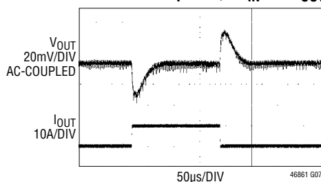
FIGURE 27 CIRCUIT AT 5\text{V}_{\text{IN}} , \text{VOUT\_COMMAND}_n SET TO 1.000\text{V} . 10\text{A} TO 20\text{A} LOAD STEP AT 10\text{A}/\mu\text{s}
