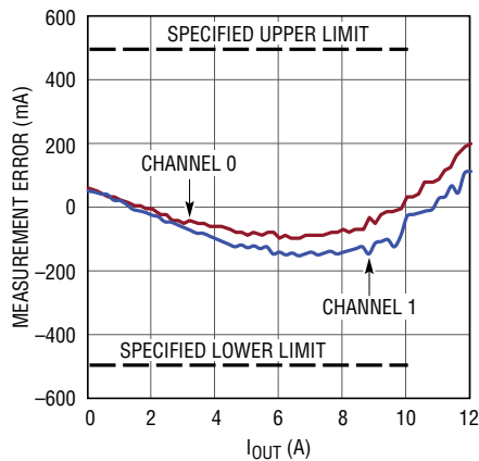
READ_IOUT n (Output Current Readback) Error vs \text{I}_{\text{OUT}n}
