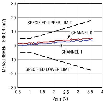
READ_VOUT n (Output Voltage Readback) Error vs \text{V}_{\text{OUT}n} \text{I}_{\text{OUT}n} = \text{No Load} , \text{RUN}_{1-n} = 0\text{V}
