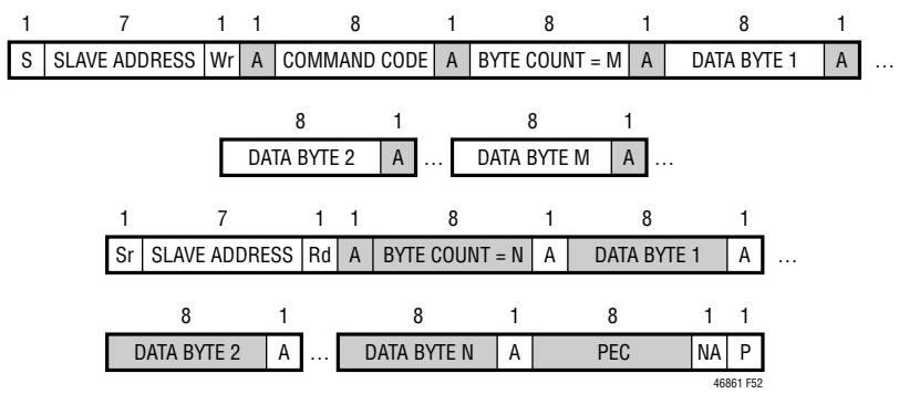
Figure 52. Block Write – Block Read Process Call with PEC
