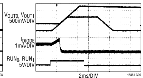
FIGURE 61 CIRCUIT AT 12\text{V}_{\text{IN}} , 100\text{m}\Omega LOAD ON \text{V}_{\text{OUT}0} , 500\Omega ON \text{V}_{\text{OUT}1} . \text{V}_{\text{OUT}1} PRE-BIASED THROUGH A DIODE. \text{TON\_RISE}_0 = 3\text{ms} , \text{TON\_RISE}_1 = 5.297\text{ms} , \text{TOFF\_DELAY}_1 = 0\text{ms} , \text{TOFF\_DELAY}_0 = 2.43\text{ms} , \text{TOFF\_FALL}_1 = 5.328\text{ms} , \text{TOFF\_FALL}_0 = 3\text{ms} , \text{ON\_OFF\_CONFIG}_1 = 0\text{x}1\text{F} , \text{ON\_OFF\_CONFIG}_0 = 0\text{x}1\text{E}
