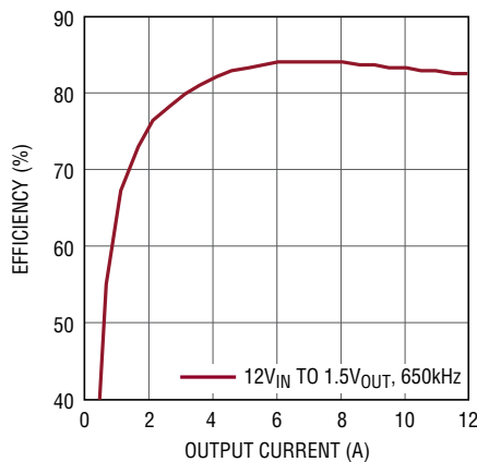
Single Phase Single Output Pulse-Skipping (Discontinuous) Mode Efficiency, V_{\text{IN}} = \text{SV}_{\text{IN}} = V_{\text{INn}} , \text{INTV}_{\text{CC}} Open, \text{MFR\_PWM\_MODE}_n[0] = 0_b
