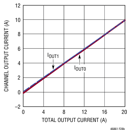
(28b) 12V IN , Figure 27 Circuit with U1 Installed with LTM4686, INTV CC Open and V OUT Commanded to 1V
