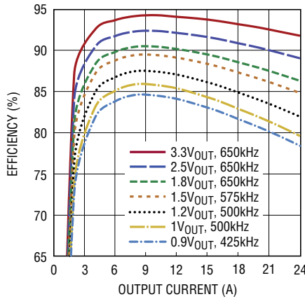
Efficiency vs Load Current at 5\text{V}_{\text{IN}}
