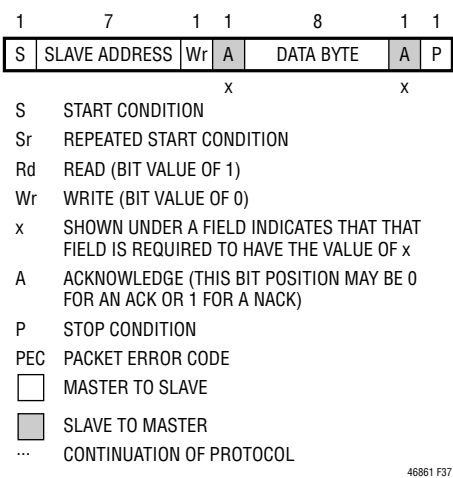
Figure 37. PMBus Packet Protocol Diagram Element Key
