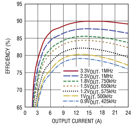
Efficiency vs Load Current at 12\text{V}_{\text{IN}}
