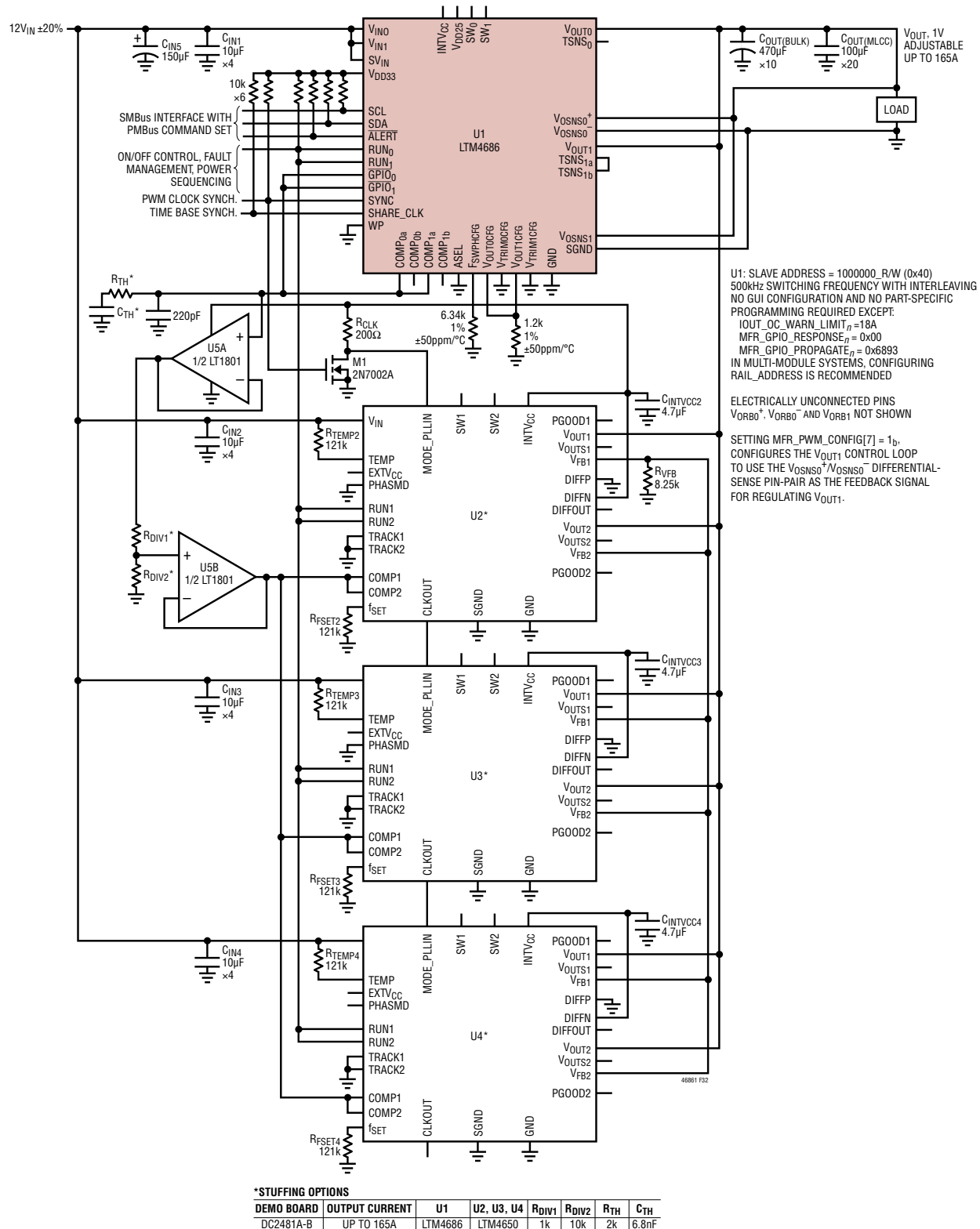
Figure 32. One LTM4686 Operating In Parallel with 3xLTM4650 (See Demo Board DC2481A-B, Custom-Stuffed with LTM4686 Module for U1) Producing 1V OUT at up to 165A. Power System Management Features Accessible Through LTM4686. See Figure 33. Contact Sales Support for Adapting Circuit for LTM4686 Use with LTM4631, LTM4620A, LTM4630
