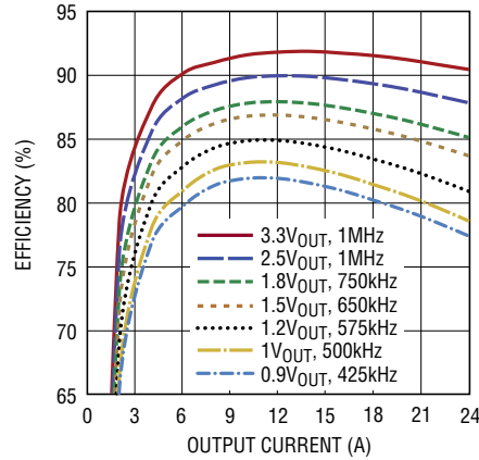
Efficiency vs Load Current at 8\text{V}_{\text{IN}}
