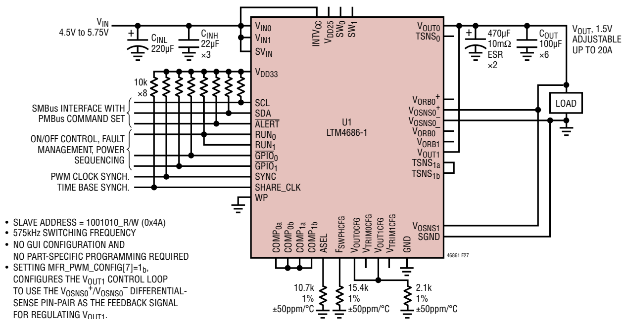
Figure 27. 20A, 1.5V Output DC/DC μModule Regulator with I 2 C/SMBus/PMBus Serial Interface
