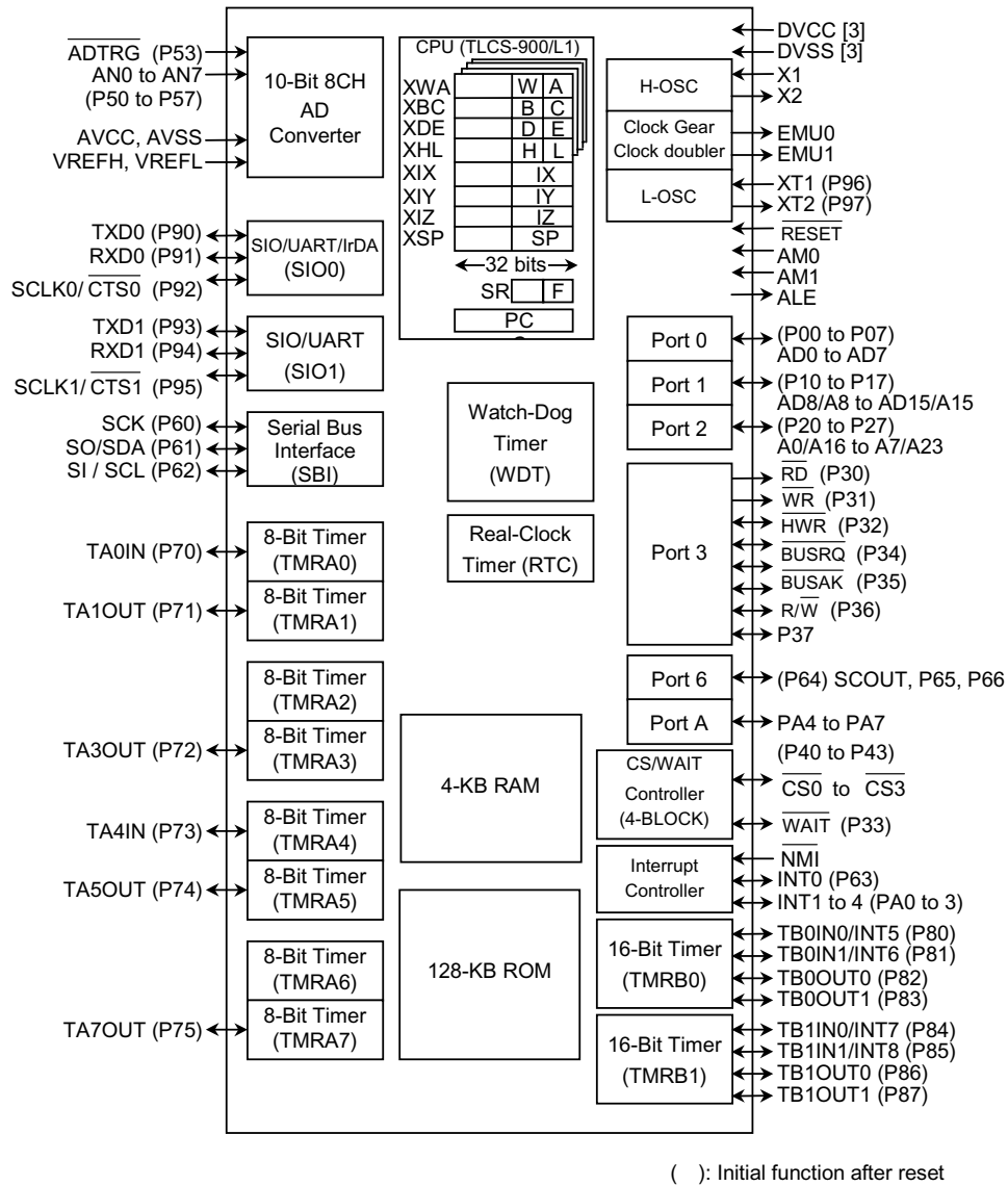
Figure 1.1 TMP91CW12AF Block Diagram
