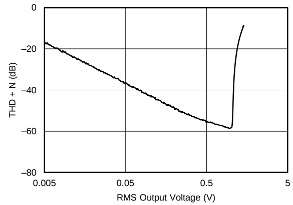
Figure 42. THD + N vs RMS Output Voltage
