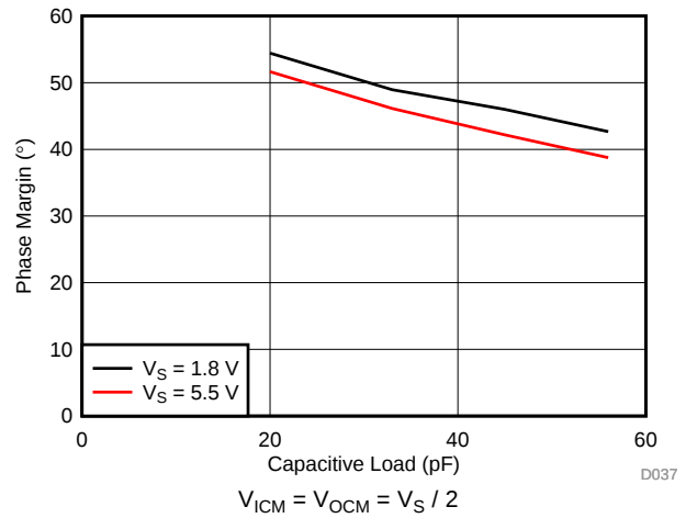
Figure 38. Phase Margin vs Capacitive Load
