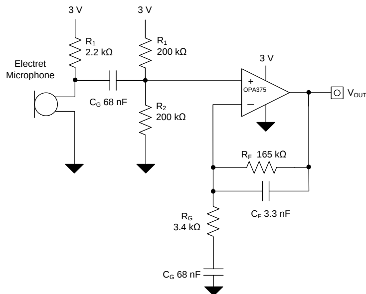
Figure 40. Microphone Pre-Amplifier
