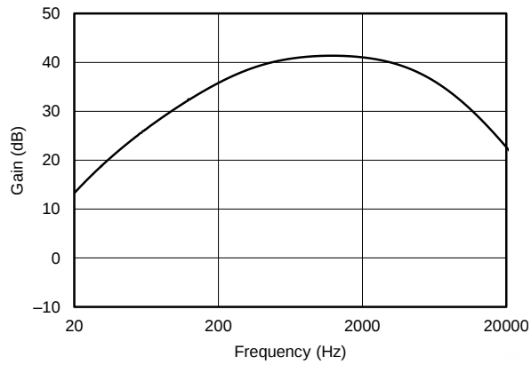
Figure 41. Gain vs Frequency
