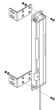
Figure 4. PVA Mounting Hardware
