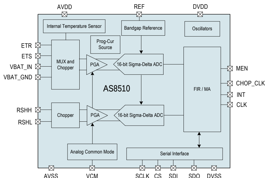
Figure 1. AS8510 Block Diagram
