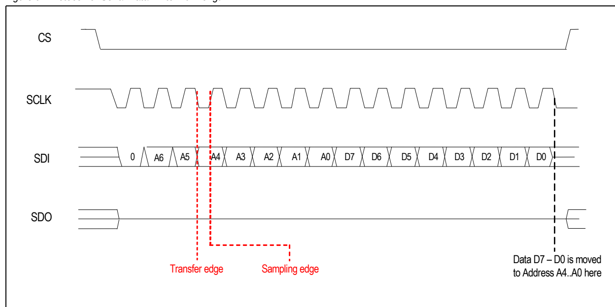
Figure 9. Protocol for Serial Data Write with Length = 1
