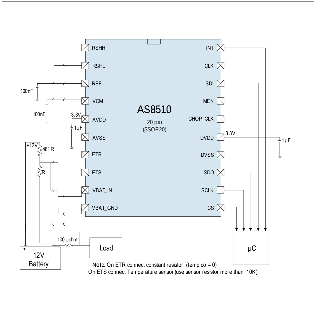
Figure 19. Application Diagram
