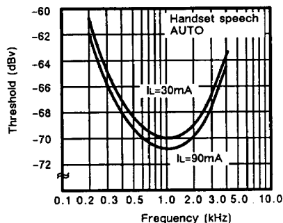
Fig. 22 - VOICE SWITCH THRESHOLD VS. FREQUENCY
