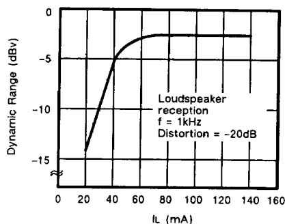
Fig. 20 - SPEAKER DYNAMIC RANGE VS. SUPPLY CURRENT
