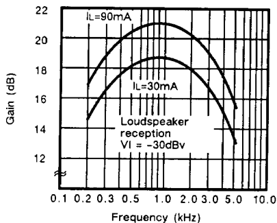
Fig. 19 - SPEAKER TOTAL GAIN VS. FREQUENCY
