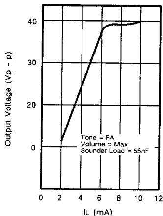
Fig. 29 - TONE RINGER OUTPUT VOLTAGE VS. SUPPLY CURRENT
