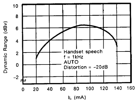
Fig. 14 - TRANSMIT DYNAMIC RANGE VS. SUPPLY CURRENT
