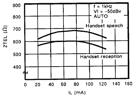
Fig. 11 - TELEPHONE AC IMPEDANCE VS. SUPPLY CURRENT
