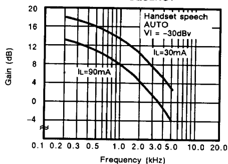
Fig. 16 - RECEPTION TOTAL GAIN VS. FREQUENCY
