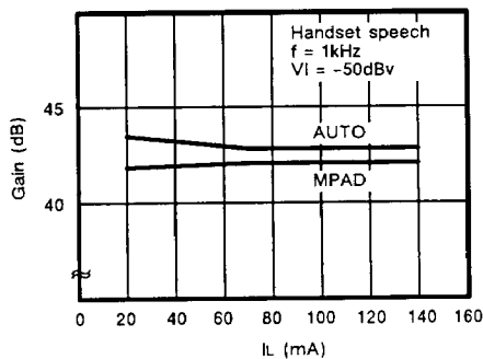
Fig. 12 - TRANSMIT TOTAL GAIN VS. SUPPLY CURRENT
