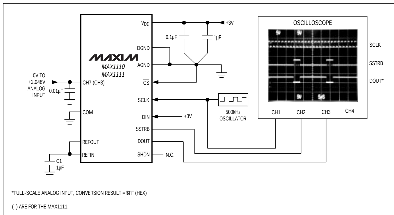
Figure 5. Quick-Look Circuit
