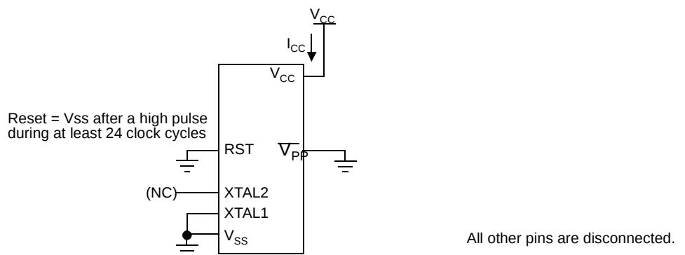
Figure 20. I_{CC} Test Condition, Power-Down Mode
