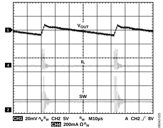
Figure 27. Steady State at Light Load, f_{\text{SW}} = 1.4\text{MHz} , I_{\text{OUT}} = 40\text{mA}
