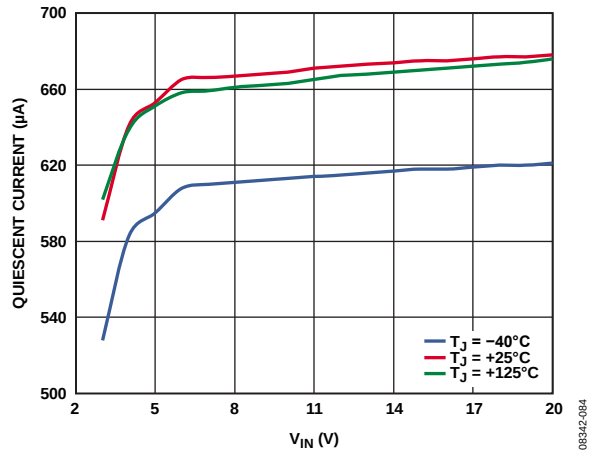
Figure 22. Quiescent Current vs. V_{\text{IN}}
