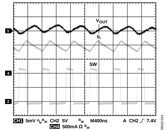
Figure 26. Steady State at Heavy Load, f_{\text{SW}} = 1.4\text{MHz} , I_{\text{OUT}} = 1\text{A}
