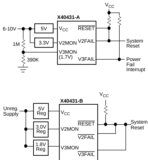
Figure 2. Two Uses of Multiple Voltage Monitoring
