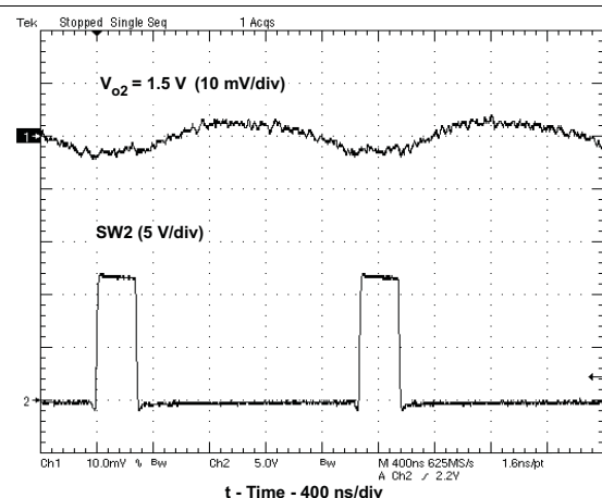
Figure 22. V OUT2 Ripple Voltage
