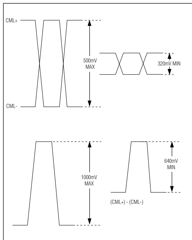
Figure 2. CML Output Levels
