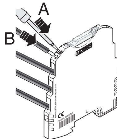
Figure 5 Spring-cage connection
