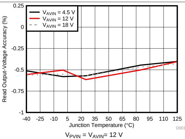
图 16. READ_VOUT Accuracy vs Junction Temperature
