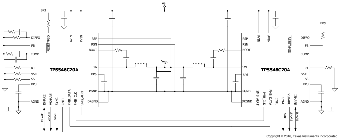
图 23. 2-Phase Application
