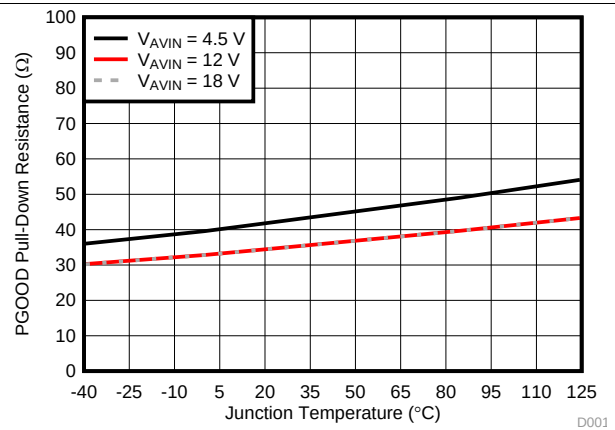
图 12. PGOOD Pulldown Resistance vs Junction Temperature
