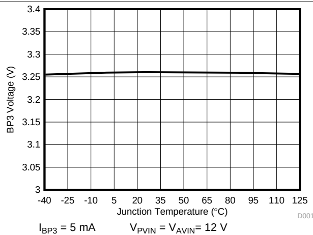
图 11. BP3 Voltage vs Junction Temperature
