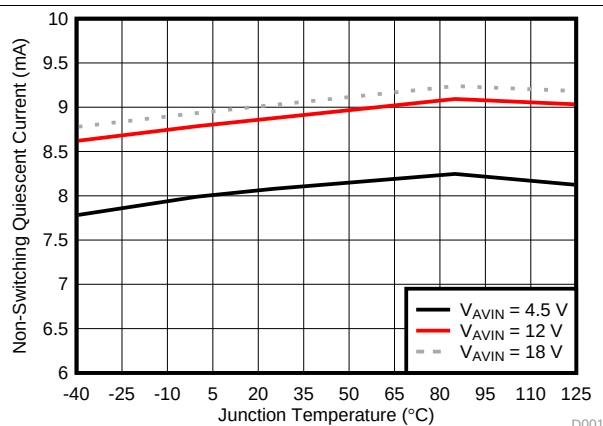
图 9. Non-Switching Input Current ( I_{AVIN} ) vs Junction Temperature
