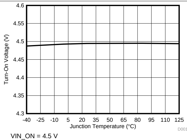
图 13. Turnon Voltage vs Junction Temperature
