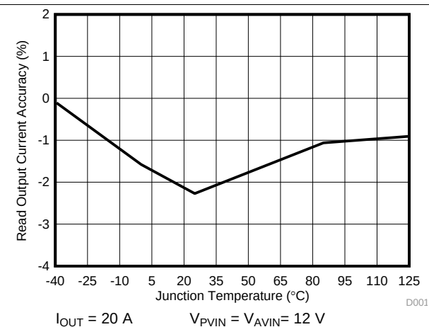
图 15. READ_IOUT Accuracy vs Junction Temperature
