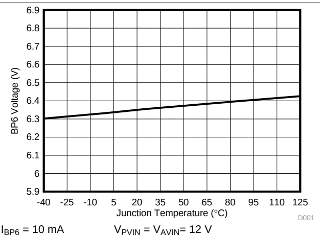
图 10. BP6 Voltage vs Junction Temperature
