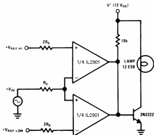
Limit Comparator
