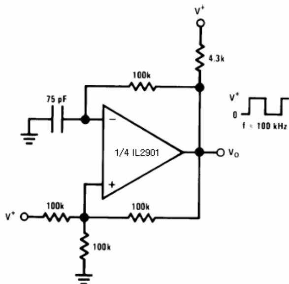
Squarewave Oscillator
