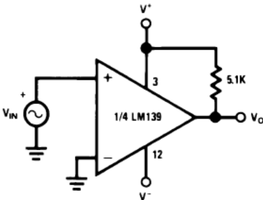
Zero Crossing Detector
