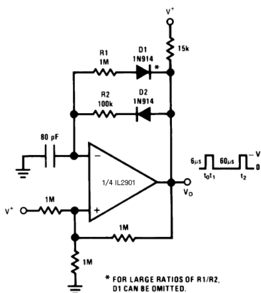
Pulse Generator
