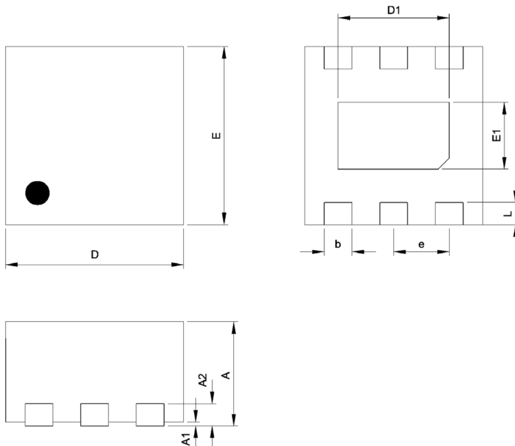
DFN1.6X1.6-6 Package
