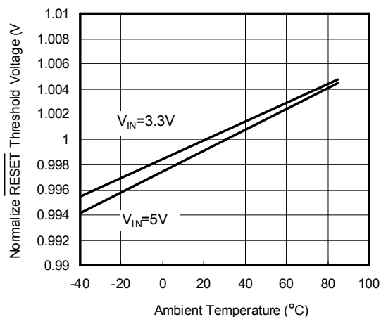
Normalize \overline{\text{RESET}} Threshold Voltage vs. Ambient Temperature
