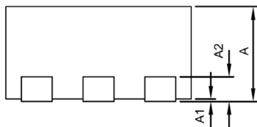
ADFN1.5X1.5-6 Package
