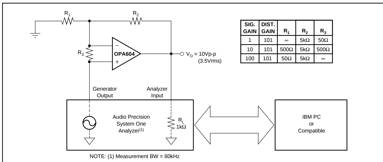
FIGURE 2. Distortion Test Circuit.
