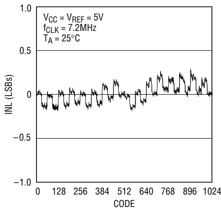
INL Plot
