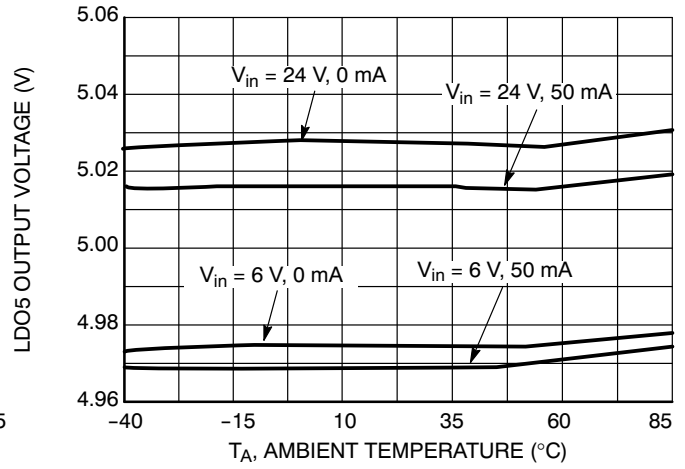
Figure 5. LDO5 Output Voltage vs. Ambient Temperature
