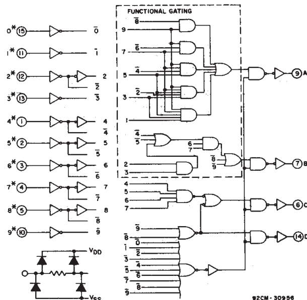
Fig. 1 - CD40147B logic diagram.
