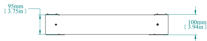
FRONT VIEW
