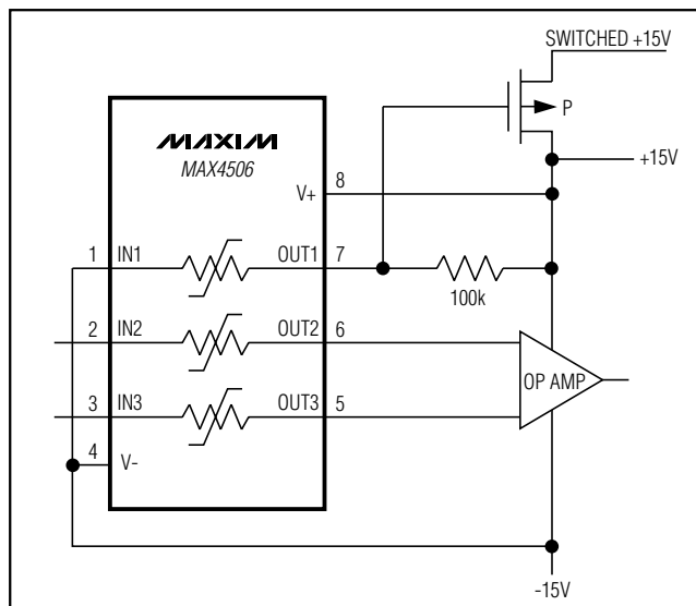
Figure 4. Power-Supply Sequencing
