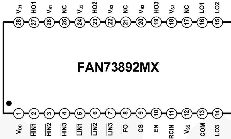
Figure 3. Pin Assignments
