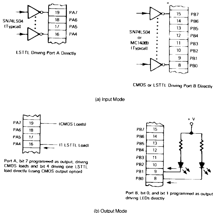
Figure 5.2 : Typical Port Connections.
