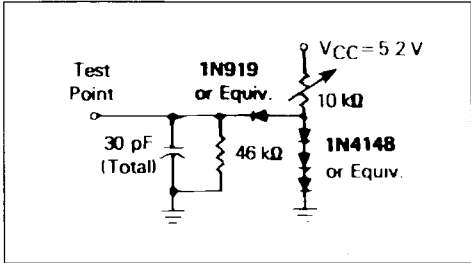
Figure 7.1 : LSTTL Equivalent Test Load (port B).
