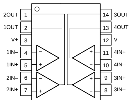
Pin Functions
