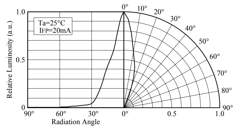
■ Directivity
