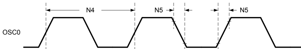
Figure 31-35. Single-Ended MOSC Characteristics for Ethernet
