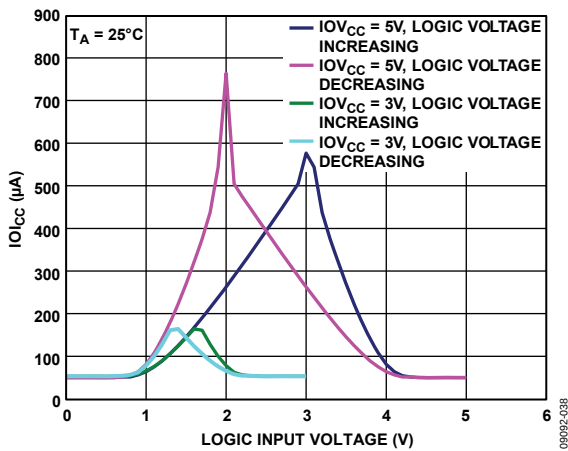
Figure 37. I_{OI} vs. Logic Input Voltage
