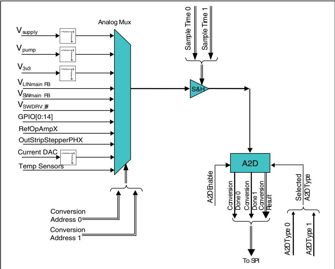
Figure 24. A2D block diagram
