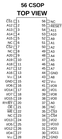
FIG. 1 PIN CONFIGURATION FOR WF4M16-XDTX5
