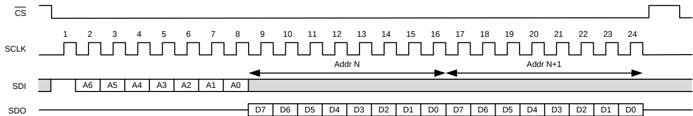
Figure 52. SPI Streaming Read Example
