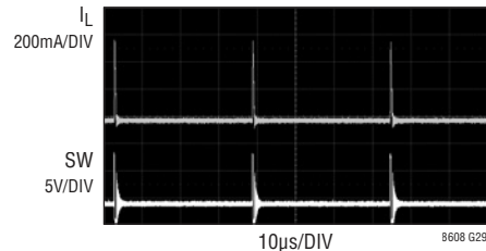
Switching Waveforms
