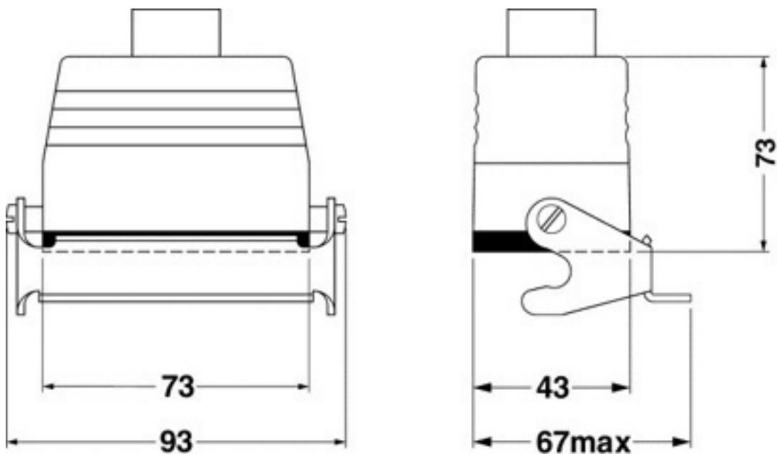
Dimensioned drawing
