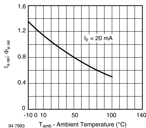
Fig. 3 - Relative Radiant Intensity / Power vs. Ambient Temperature
