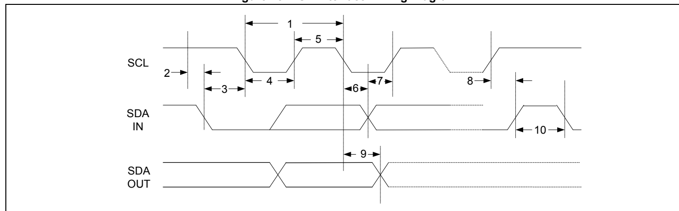
Figure 18. BSC Interface Timing Diagram
