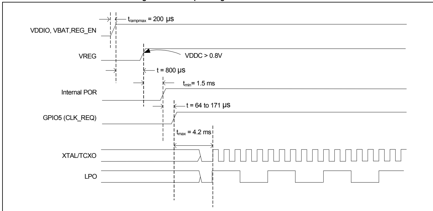
Figure 11. Startup Timing from Power-on Reset
