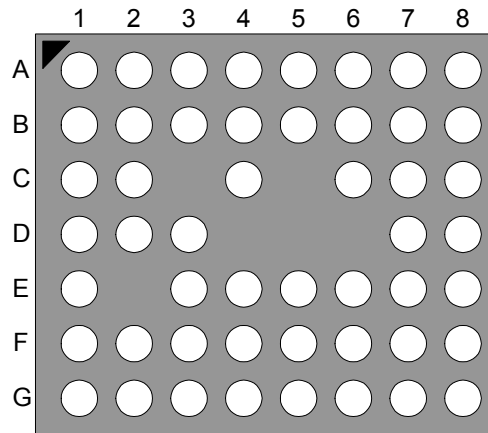
Figure 9. 4.5 x 4 x 0.8 mm (WFBGA) Arra
