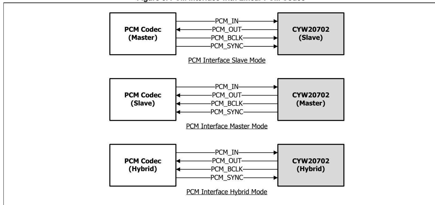
Figure 5. PCM Interface with Linear PCM Codec
