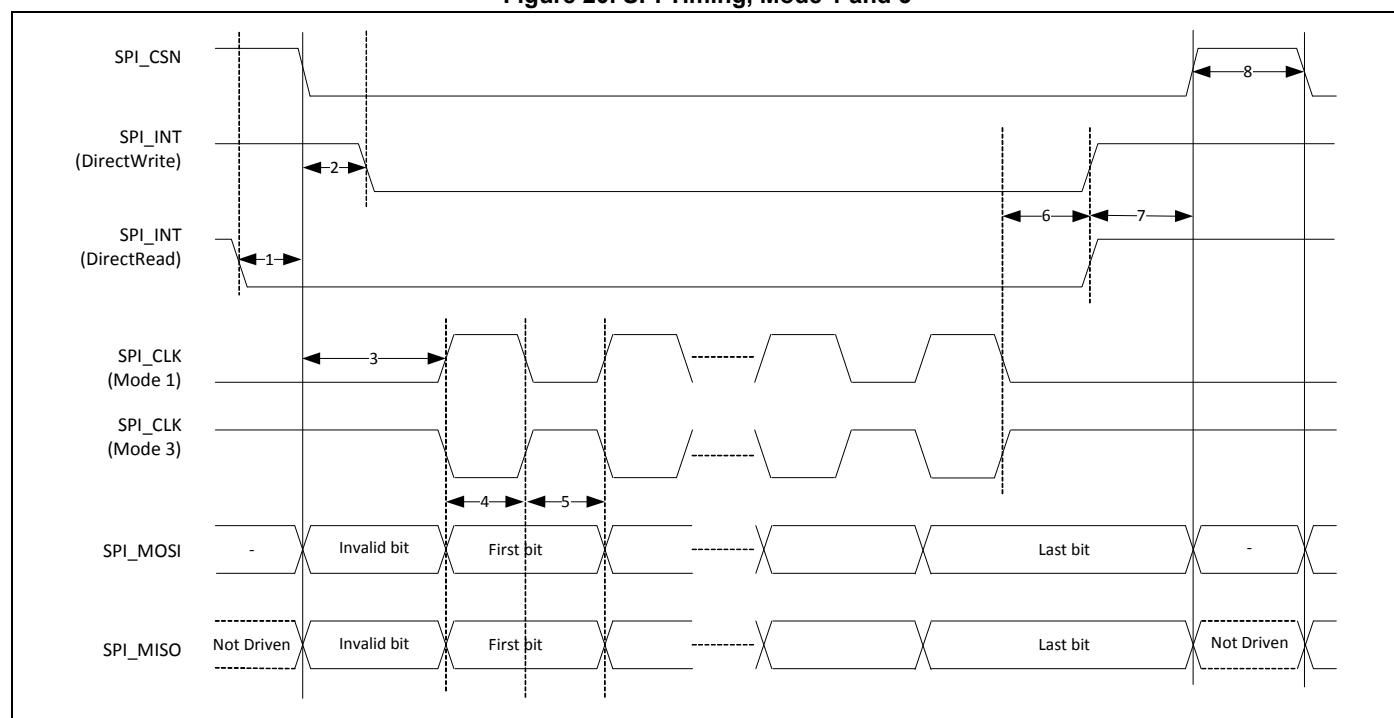
Figure 20. SPI Timing, Mode 1 and 3
