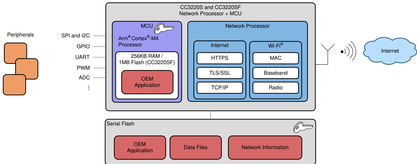
图 9-2. CC3220S and CC3220SF High-Level Structure
