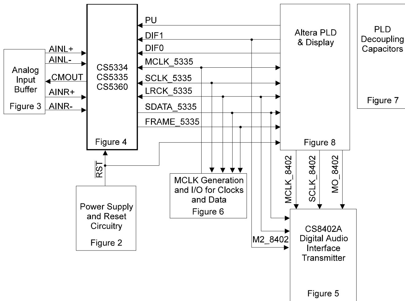
Figure 1. System Block Diagram and Signal Flow
