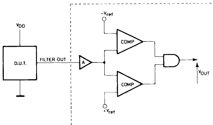
Figure 1 : DC + AC Out Level Measurement Test Set.
