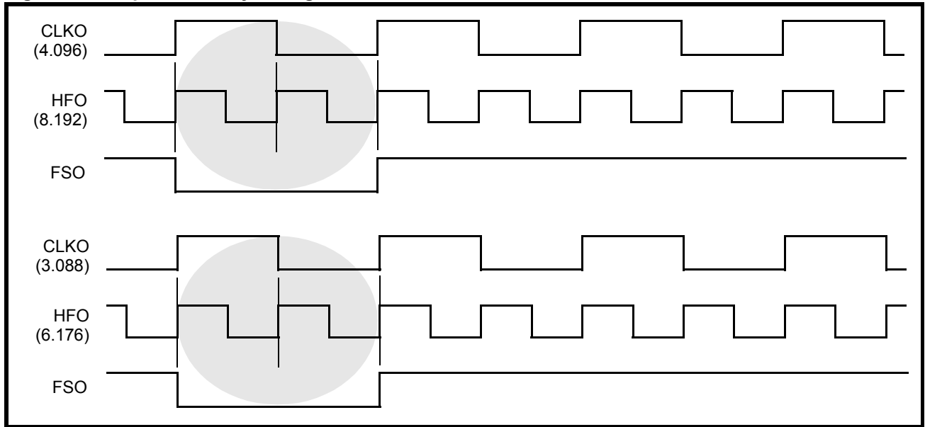
Figure 8: Output Frame Sync Alignment when HFO = 2 \times CLKO
