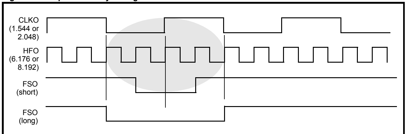
Figure 10: Output Frame Sync Alignment when HFO = 4 \times CLKO
