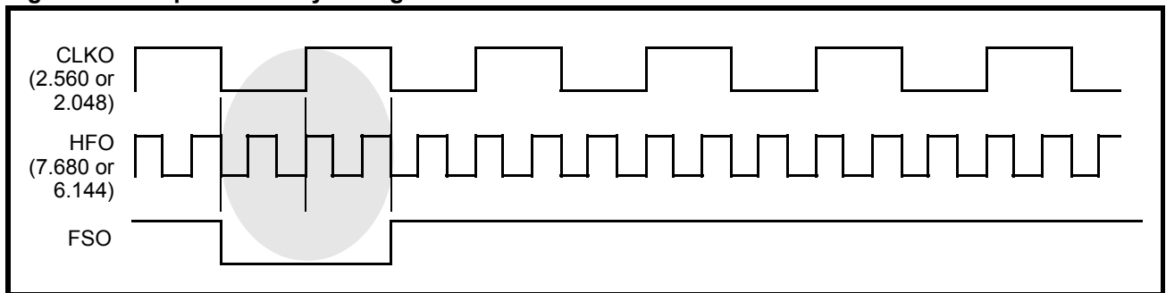
Figure 9: Output Frame Sync Alignment when HFO = 3 \times CLKO
