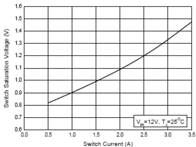
Figure 8. Switch Saturation Voltage vs. Switch Current
