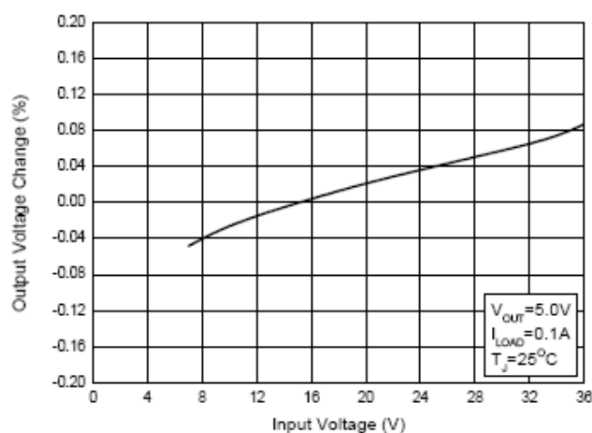
Figure 6. Line Regulation
