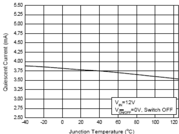
Figure 11. Quiescent Current Limit vs. Junction Temperature
