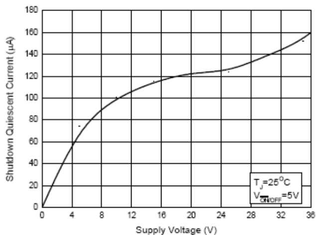
Figure 12. Shutdown Quiescent Current vs. Input Voltage
