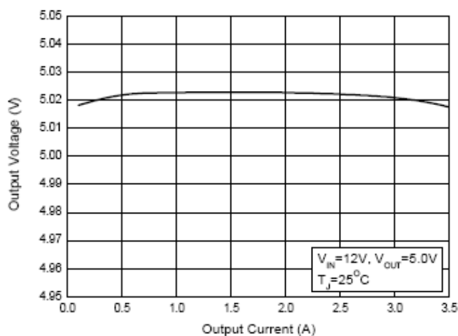
Figure 7. Load Regulation
