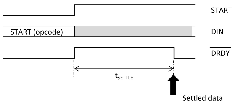
Figure 24. Settling Time For Initial Conversion
