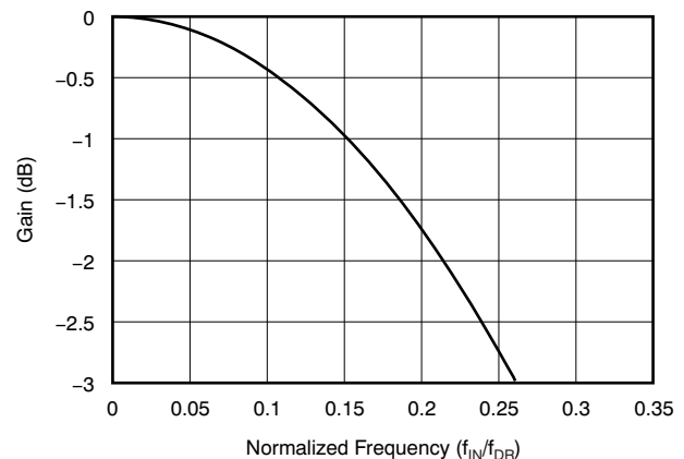
Figure 34. Sinc Filter Roll-Off
