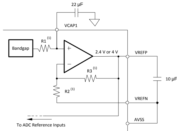
Figure 44. Internal Reference
