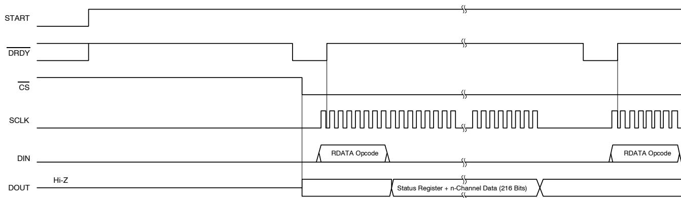
Figure 20. RDATA Usage
