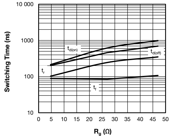
Fig. 14 - Typical IGBT Switching Time vs. R_g T_J = 125\text{ }^\circ\text{C} , V_{CC} = 325\text{ V} , I_C = 200\text{ A} , V_{GE} = 15\text{ V} , L = 500\text{ }\mu\text{H}
