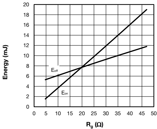
Fig. 13 - Typical IGBT Energy Loss vs. R_g T_J = 125\text{ }^\circ\text{C} , V_{CC} = 325\text{ V} , I_C = 200\text{ A} , V_{GE} = 15\text{ V} , L = 500\text{ }\mu\text{H}
